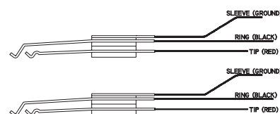
Non-Normalled
