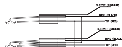
Half-Normalled
