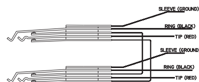
Full-Normalled
