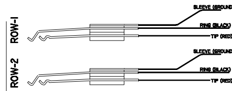
T,R,S OUT NON-NORMALLED TYPE 3
