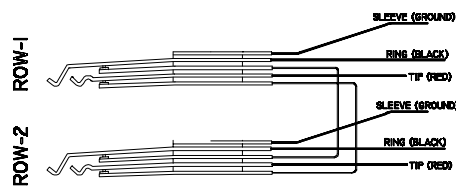
FULL NORMALLED TYPE 1
