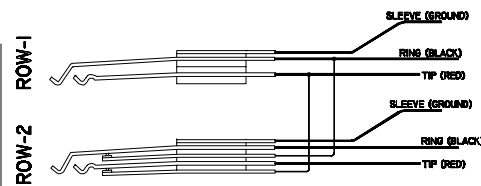
T,R,S OUT HALF-NORMALLED TYPE 2
