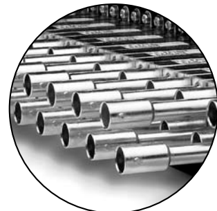
Rear view (32MV2/MVJ-3T) Mid-size Video Patchbay showing staggered BNC termination.
