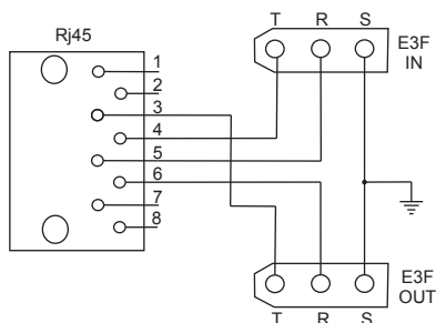
RTS Wiring Diagram
